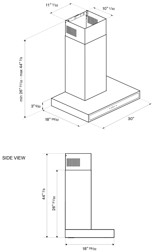
PRODUCT DIMENSIONS
